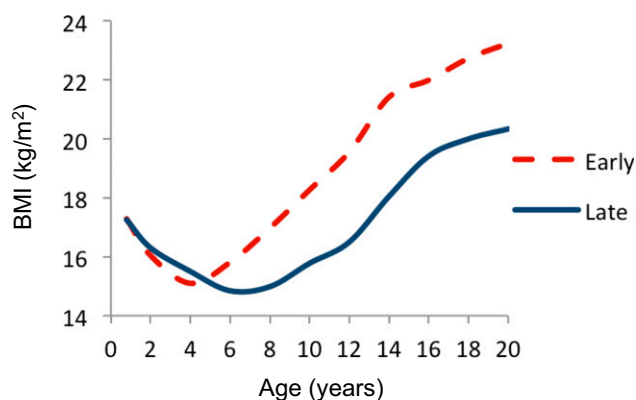
Fig. 1. Developmental changes in BMI ( \text{kg}/\text{m}^2 ) related to age at adiposity rebound in a French study. Reprinted from ref. 96, licensed under CC BY-NC-ND 4.0.
