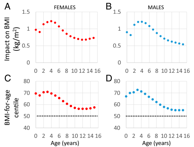
Fig. 5. The predicted impact on BMI of moving from 20% above the mean for brain energy use to 20% below the mean for brain energy use (a reduction of 33%). Median height and weight for age (CDC) were used to estimate the BMI. An estimate of additional weight gained as a result of energy saved from reduced brain expenditure was calculated using the method of Swinburn et al. (78), from which a second BMI was calculated. The plotted values are the differences between the two BMI estimates in (A) females and (B) males. The BMI centile predicted after that level of energetic savings in (C) females and (D) males (dotted lines reflect the starting point of the 50th centile).
